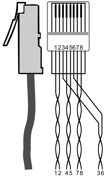
Figure 4: RJ-45 PINOUT
