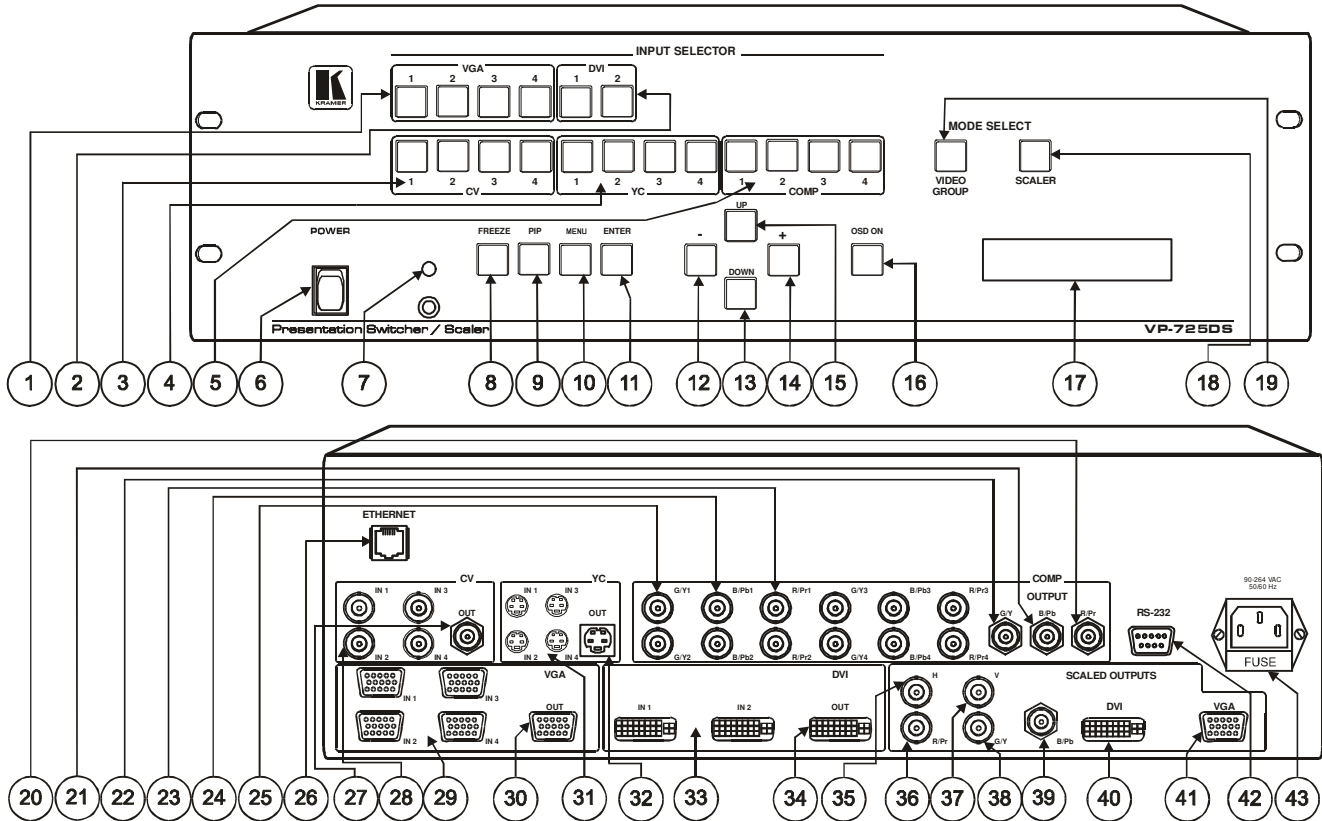
Figure 1: VP-725DS Presentation Switcher / Scaler
