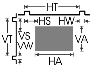
Figure 16: User Mode Setting
