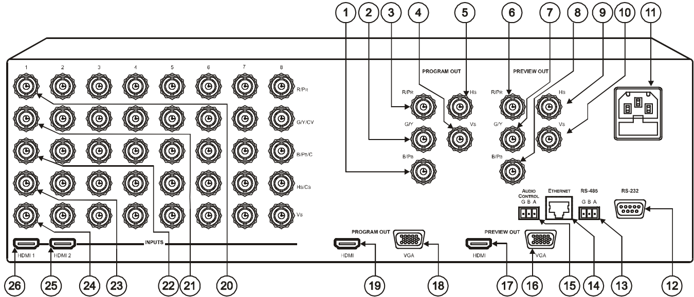
Figure 2: VP-727xl Universal Presentation Matrix Switcher / Scaler Rear Panel
