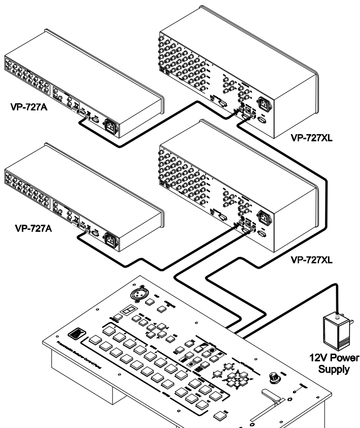
Figure 8: Connecting the VP-727T to the VP-727xl
