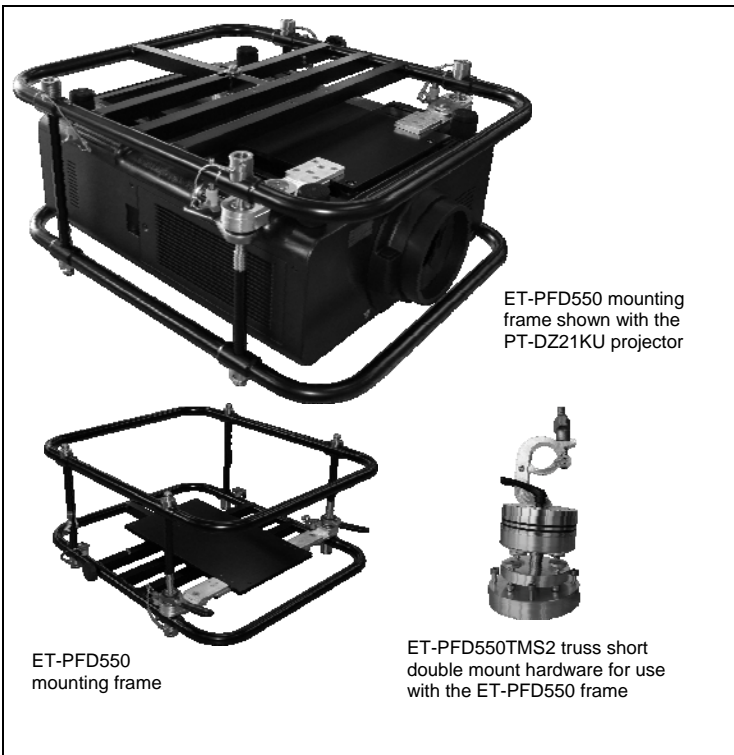
▲ ET-PFD550 shown with the ET-PFD550TMS2 truss short double mount hardware and PT-DZ21KU projector.
