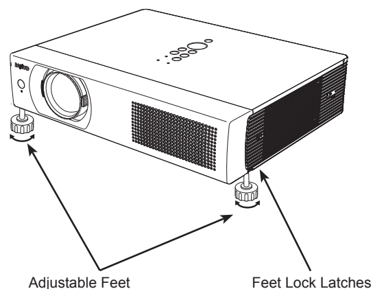
Adjustable Feet
