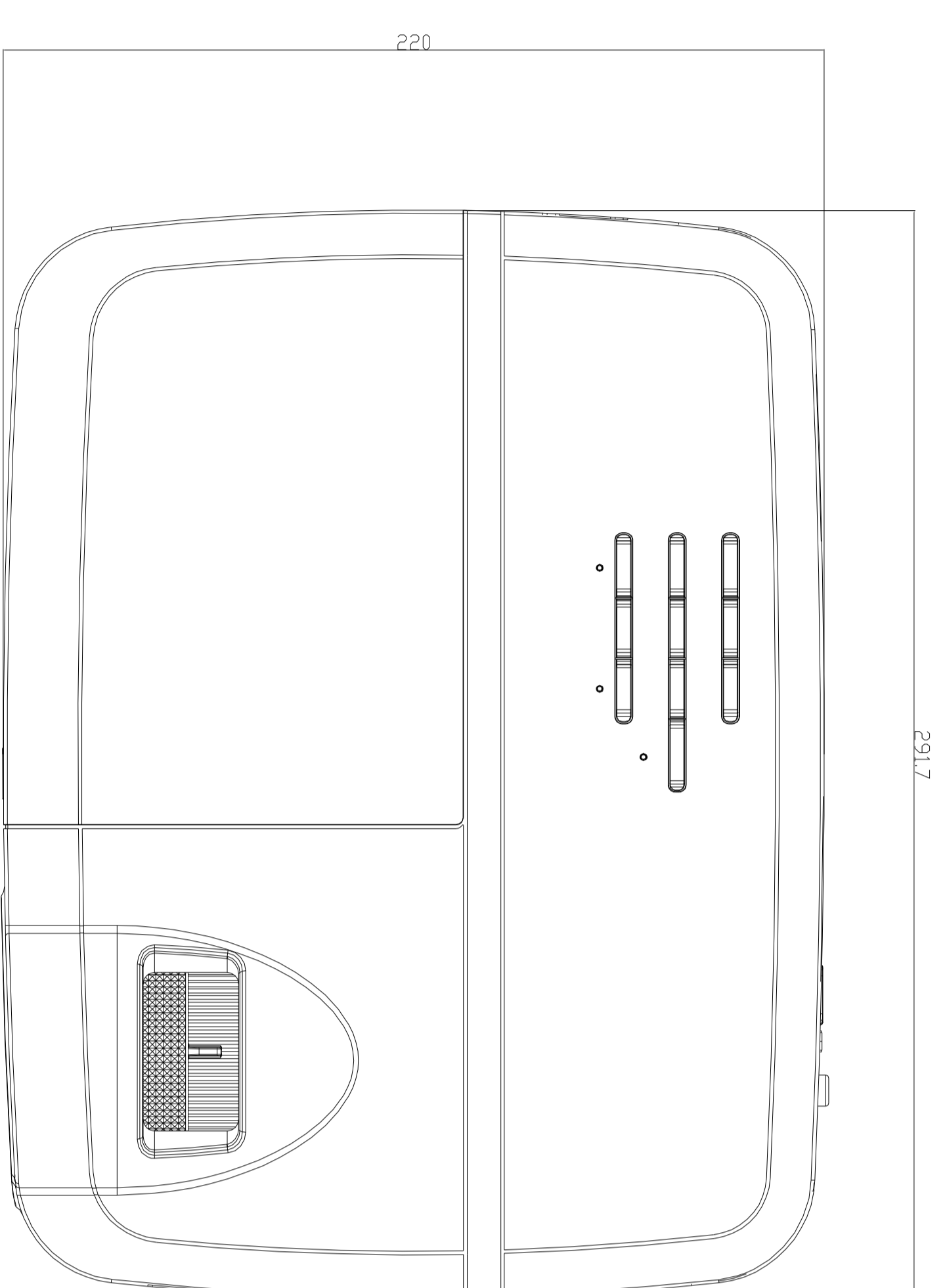
TOP VIEW
