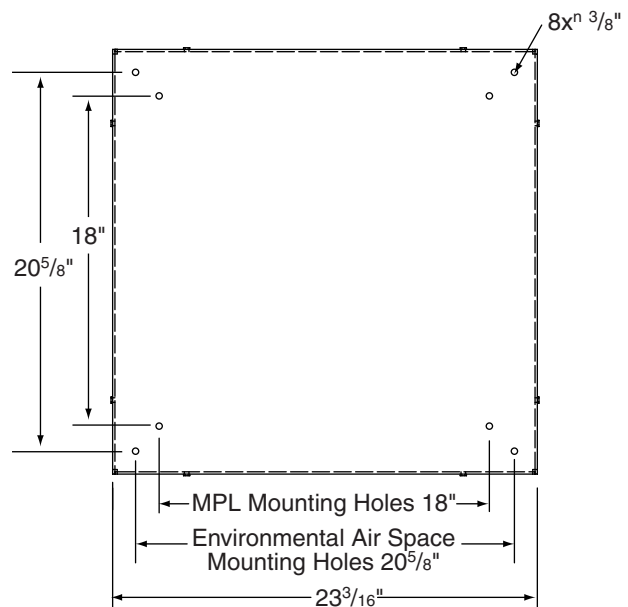
(Top view of Environmental Air Space Housing shown)
