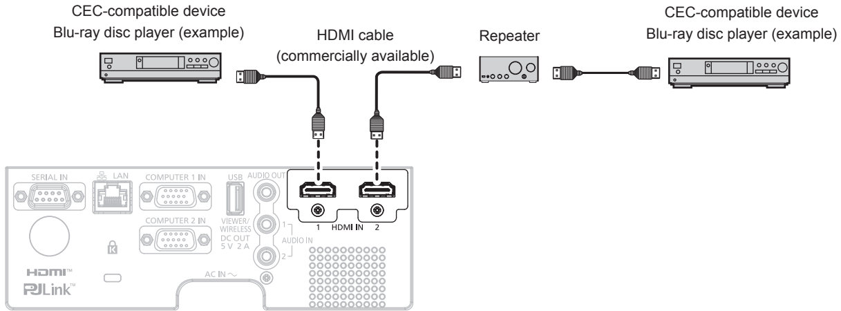
Connection example with CEC-compatible device
