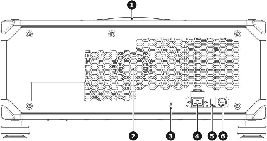
Image 2-7 Rear view
