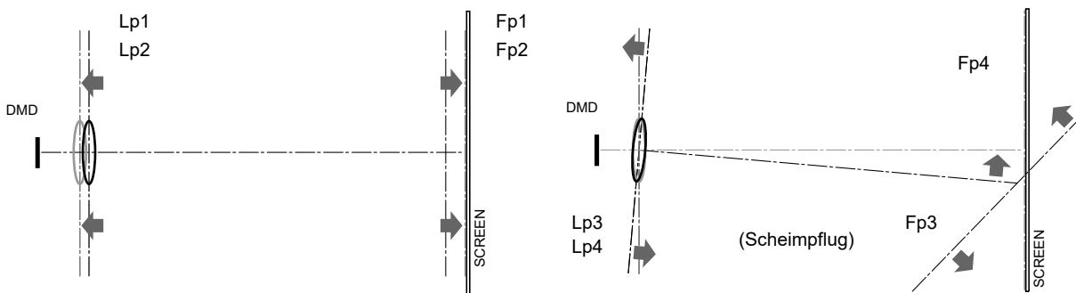
Image 3-6 Boresight (Scheimpflug) principle
