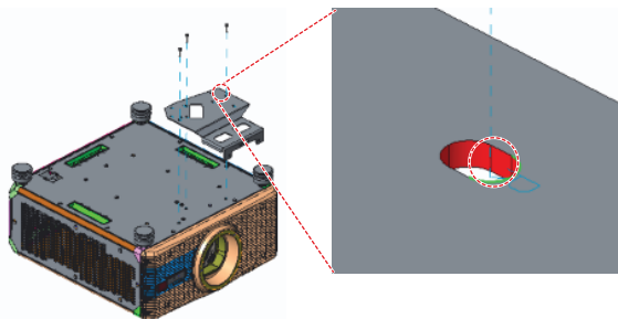
Image 5–15 Mount bottom plate on the front side of the projector
