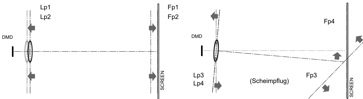
Image 5-5 Boresight (Scheimpflug) principle
