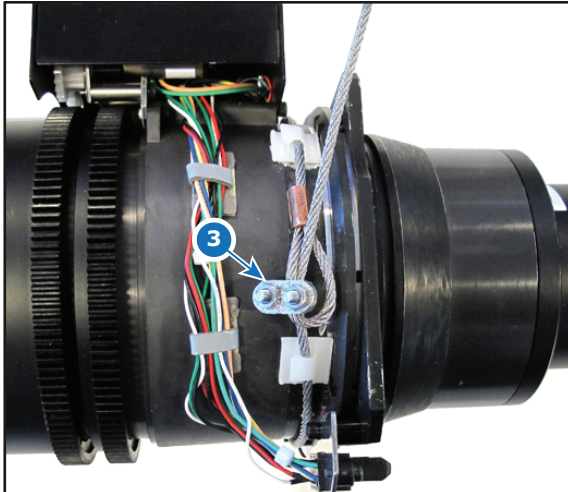
Image 3-8 Example of Configuration A
