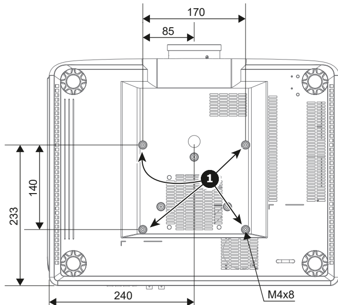
Image 3-17 Dimensions given in mm
