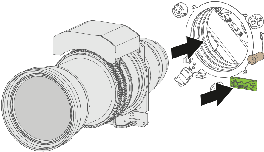
Image 4-7 Lens installation
