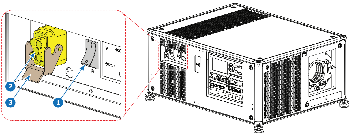
Image 4-4 Power input
