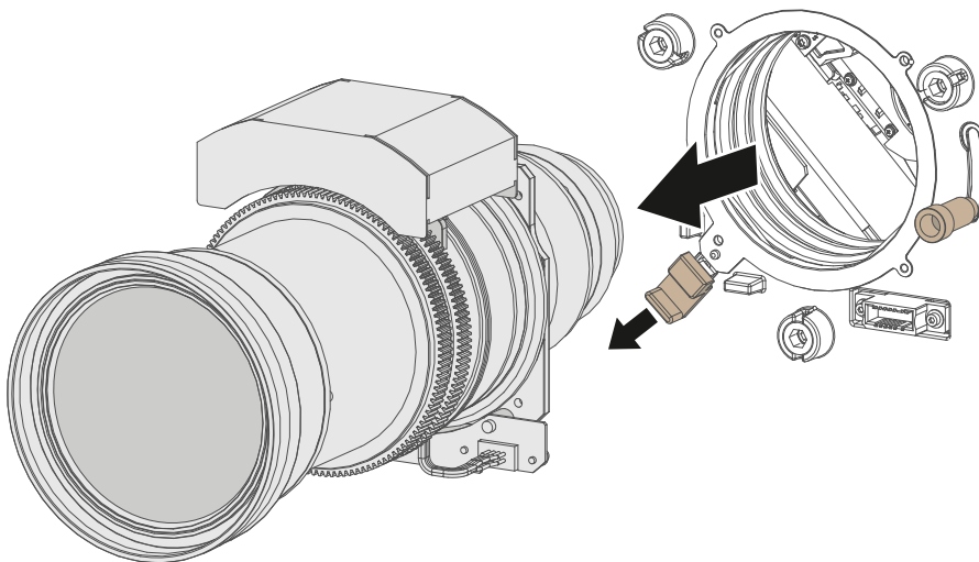
Image 4-10 Lens removal
