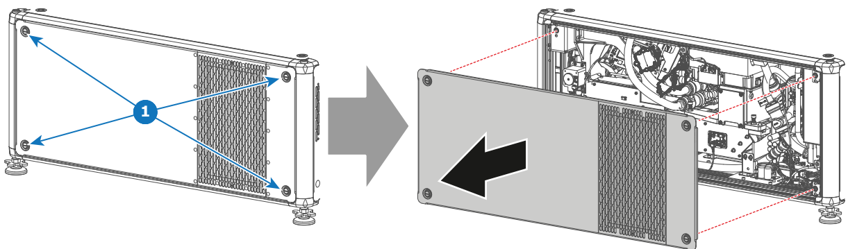
Image 8-2 Removal of the left cover (light processor side)
