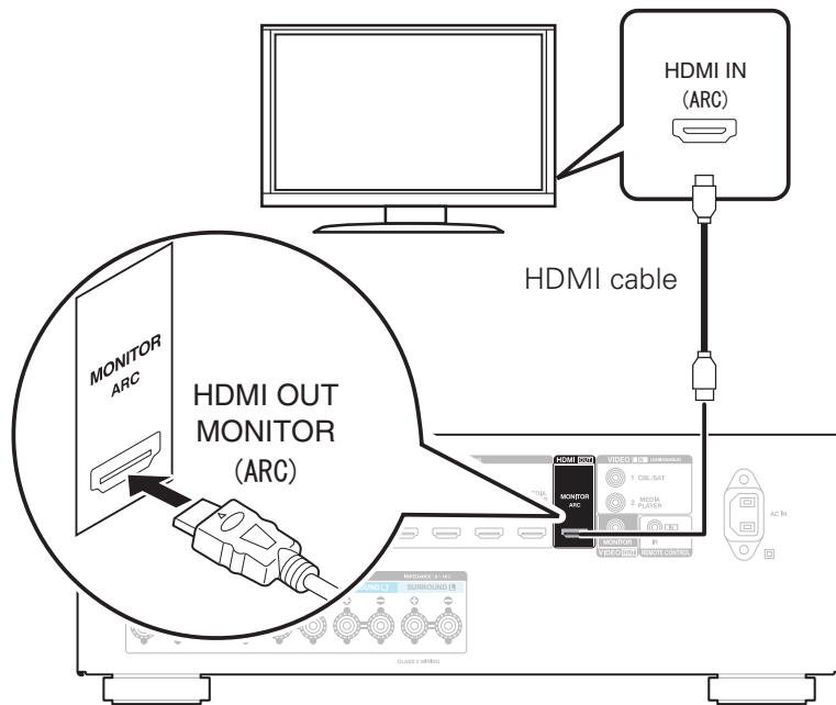
Receiver (Rear panel)
