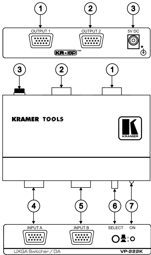
Figure 1: VP-222K UXGA Switcher / DA
