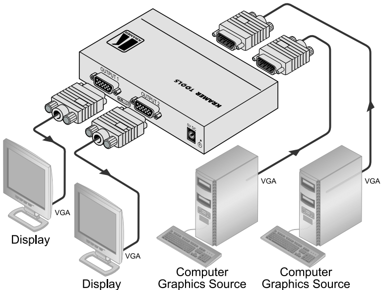
Figure 2: VP-222K UXGA Switcher / DA Connections
