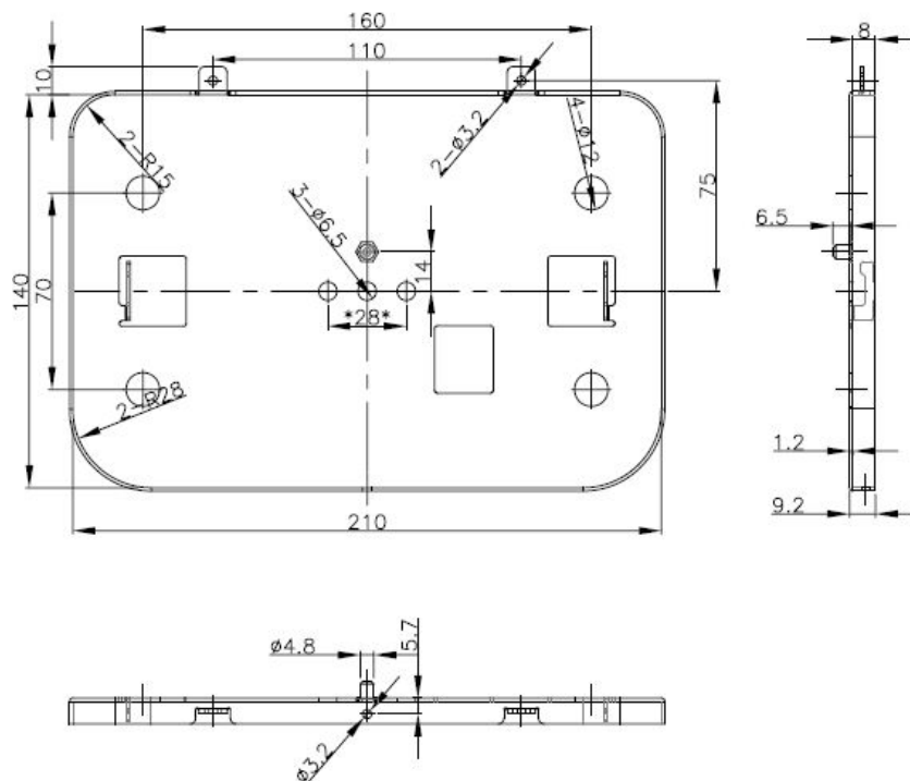
Lower cover
