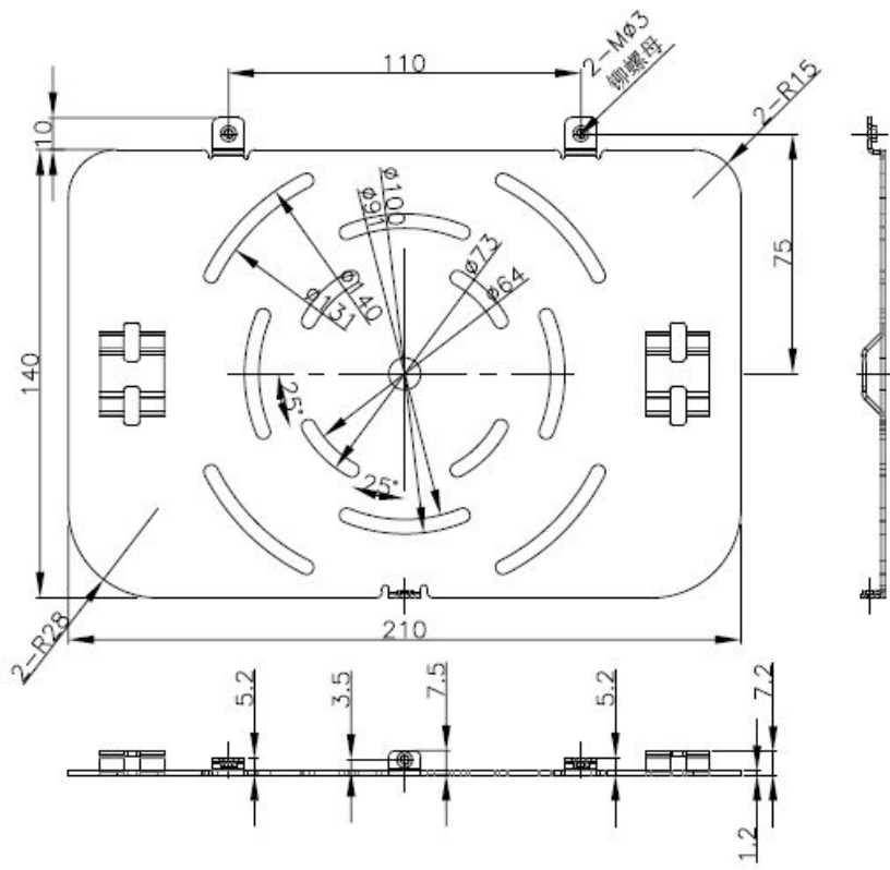
Upper cover
