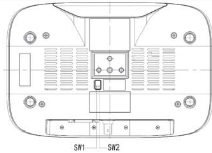
Figure 2.5 Bottom DIP Switch diagram
