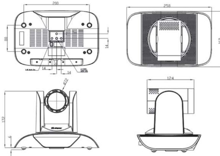
Figure 2.2 Camera dimension
