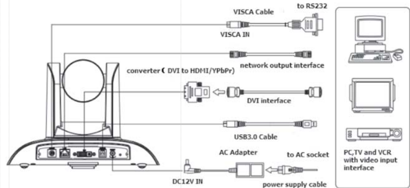
Figure 2.4 U3 model external interface diagram
