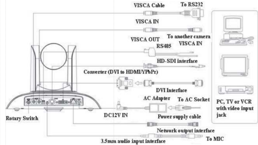
Figure 2.3 ST model external interface diagram
