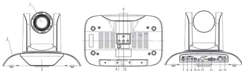
Figure 1.1 Interface of ST (standard) series
